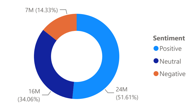
Sentiment analysis
